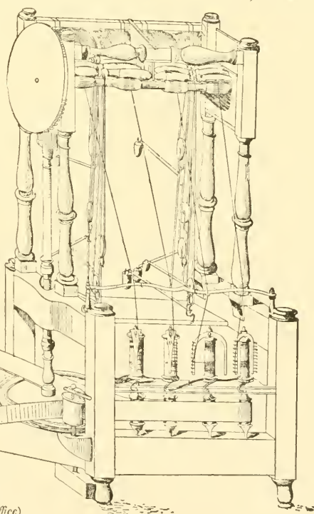
MODEL OF ARKWRIGHT'S SPINNING JENNY, 1769
